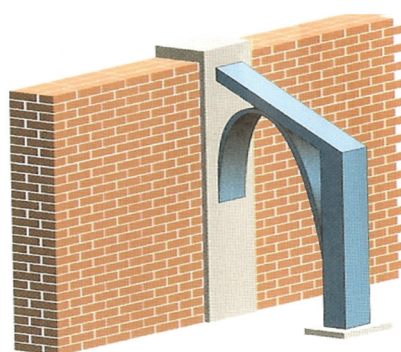
Figure 5.3.8 Schematic of attaching buttresses
