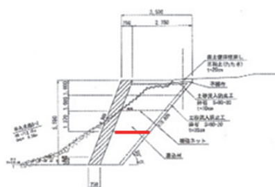
Cross-section view
