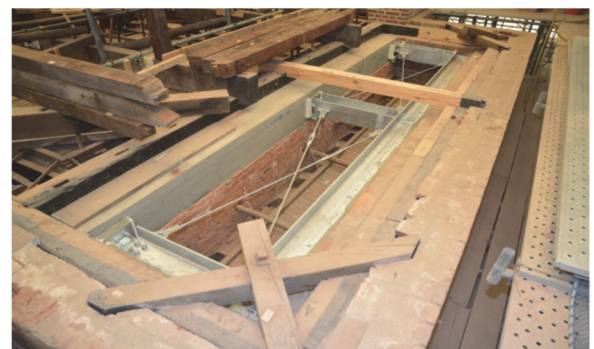
Installation of reinforced concrete (RC) beams
