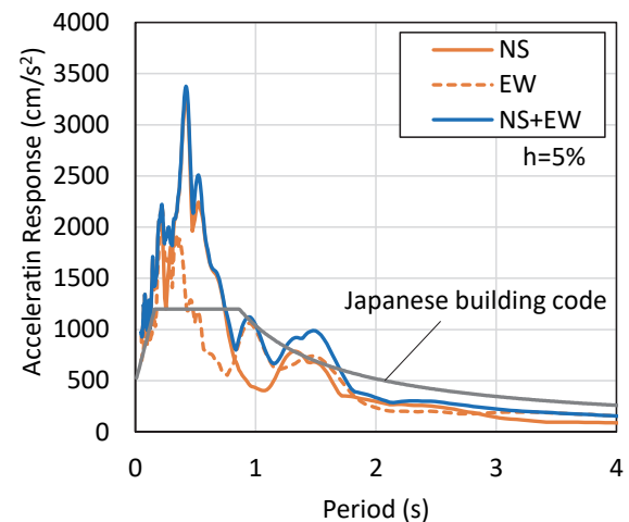
Figure 3.1.8 Acceleration response spectrum of K-net Kumamoto (KMM006) observation record
