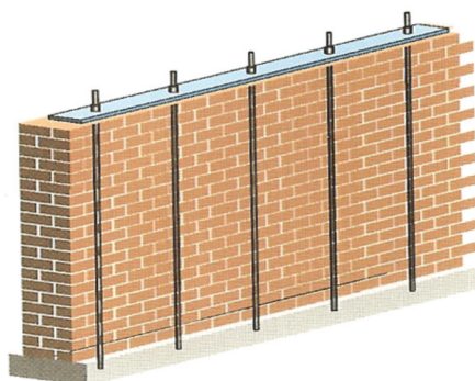
Figure 5.3.6 Schematic of prestressing method using high strength steel bars
